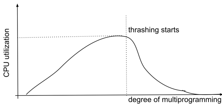
Fig 5.32: Thrashing
