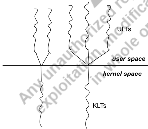
Fig 2.15: Many-to-one model
