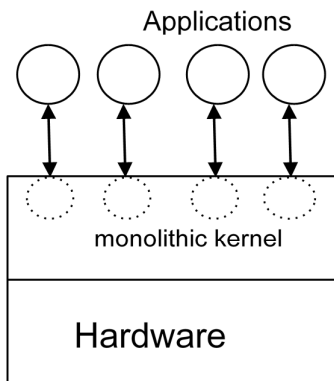
Fig 1.20: Monolithic kernel
