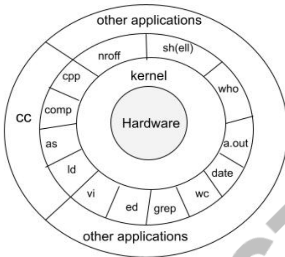
Fig 1.26: UNIX architecture
