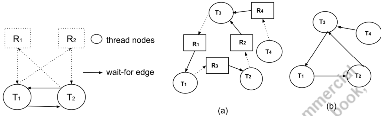
Fig 4.12: A wait-for graph (b/w T_1 & T_2 only) from Fig 4.6
