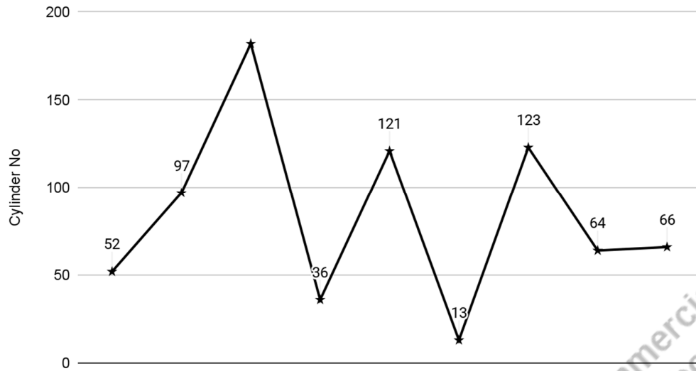
Fig 6.11: FCFS Scheduling
