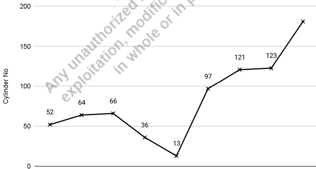
Fig 6.12: SSTF Scheduling
