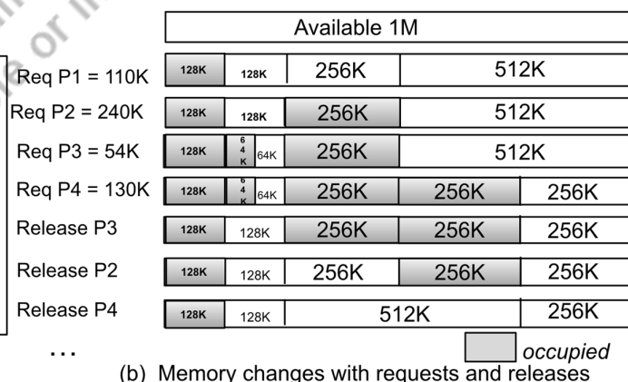
Fig 5.8: Buddy System
