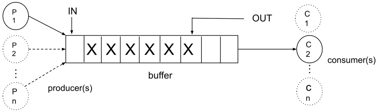
Fig 3.28: Producer-Consumer Model
