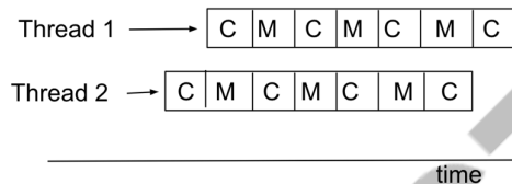
Fig 2.23: Multi-threaded core
