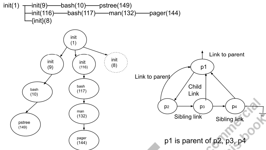
Fig 2.3: Process tree with pids (Linux command: ps tree -p )
