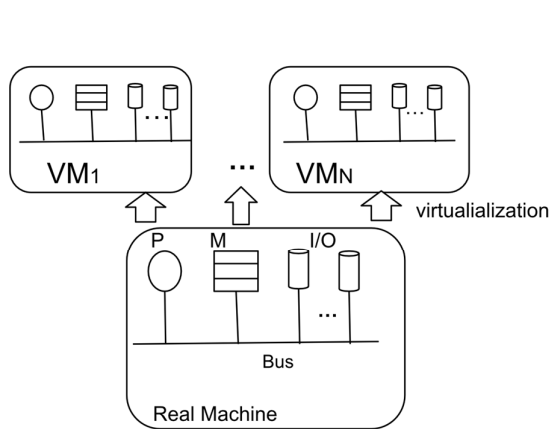
Fig 1.23: Single h/w m/c virtualized to multiple virtual m/cs (system-level virtualization)
