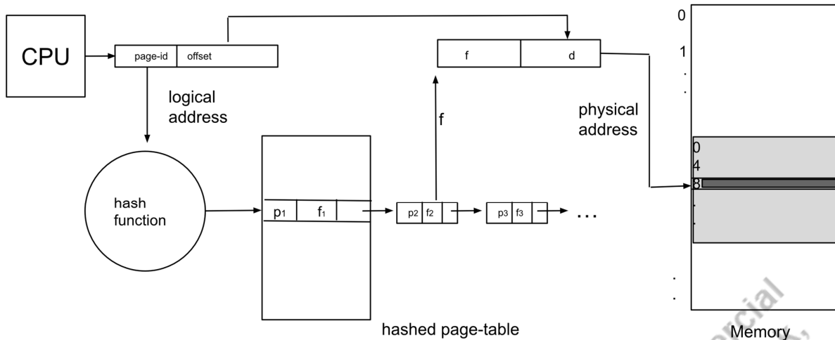
Fig 5.13: Address translation with hashed page-table
