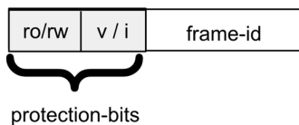
Fig 5.15: An entry in a page table
