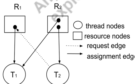
Fig 4.7: A RAG with multiple instances of resources
