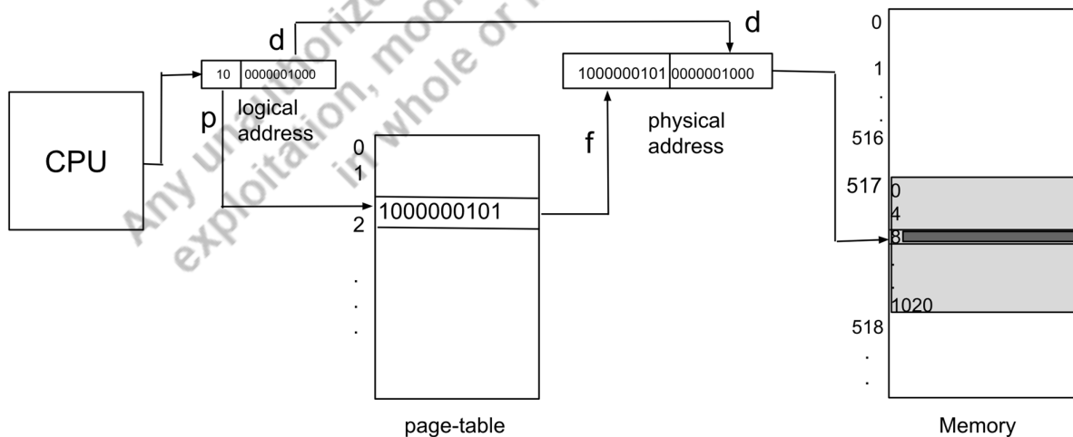
Fig 5.9: Address translation in paging using a page-table
