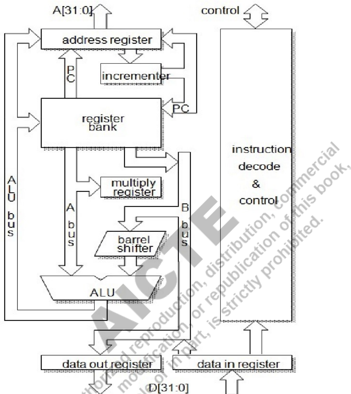
Fig. 6.18: ARM 6 Architecture [Courtesy: ResearchGate]
