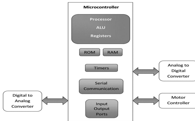
Fig.1.4: Basic architecture of Microcontroller
