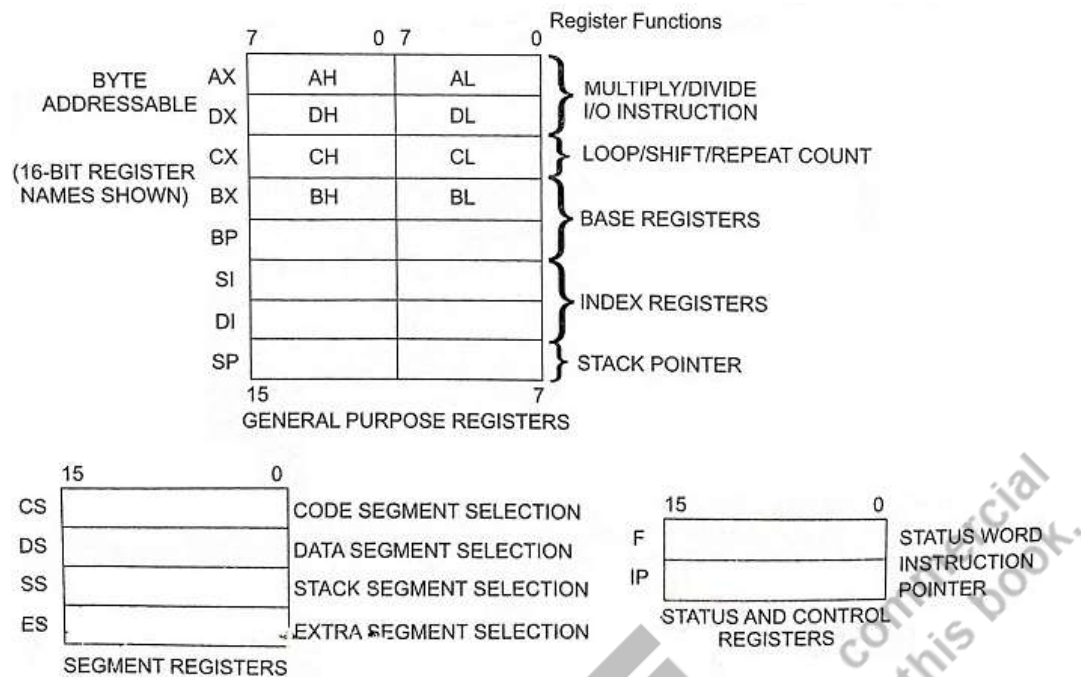
Fig. 6.4: Register Set of 80286 Processor [Courtesy: EEGUIDE]
