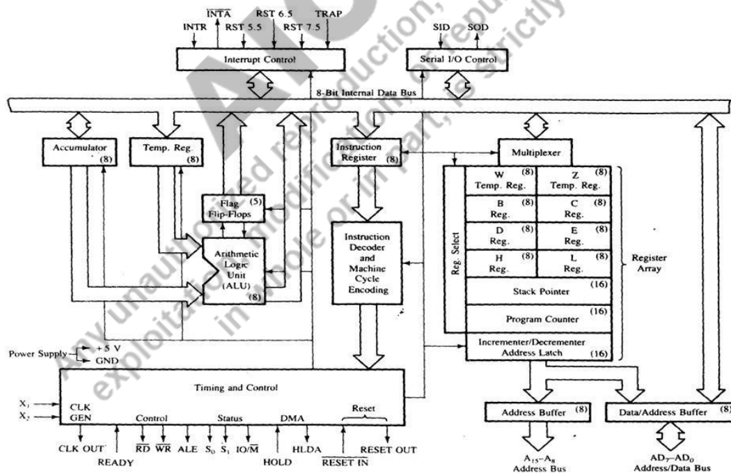
Fig. 1.8: Architecture of 8085
