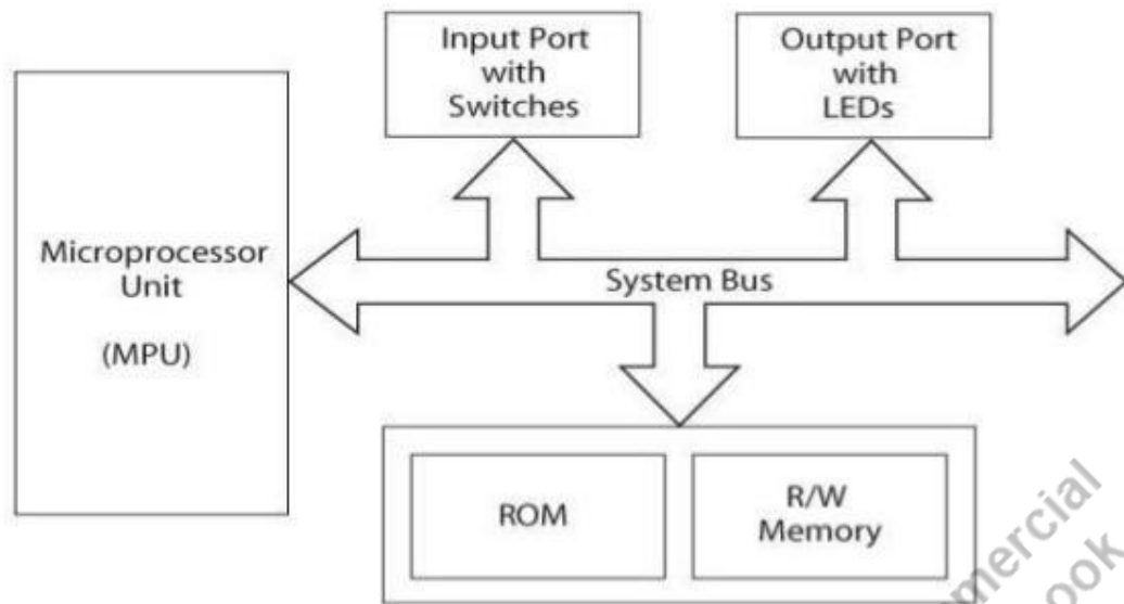
Figure 1.5: General organization of a Microprocessor based System
