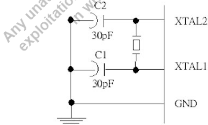
Fig. 2.7: Clocking Circuit (Crystal Oscillator) of 8051
