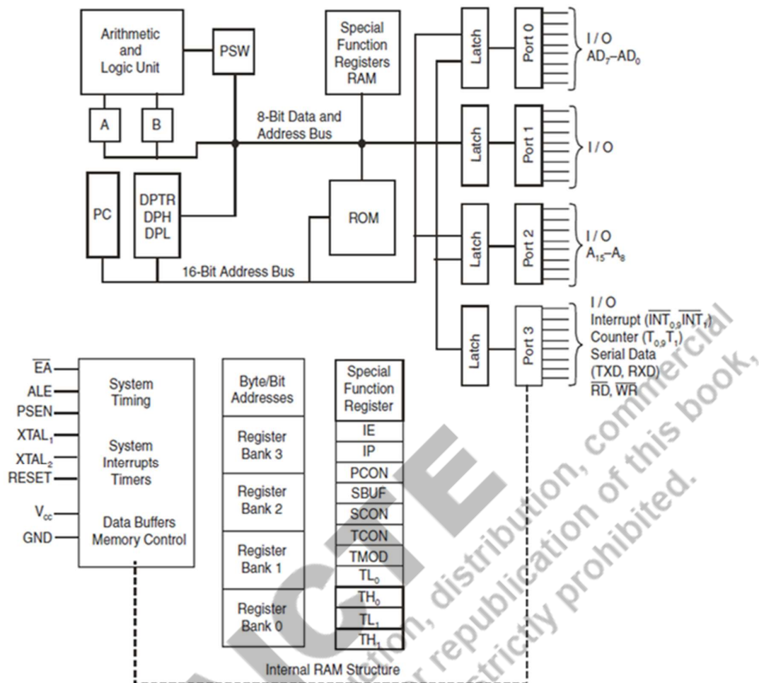
Fig.2.2: Detailed block diagram of 8051 microcontroller with internal registers
