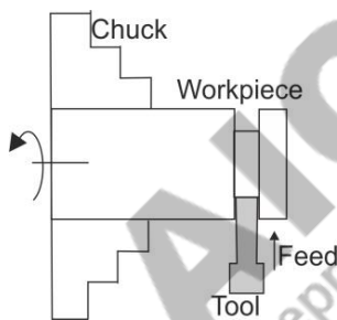
Fig. 5.9: Parting
