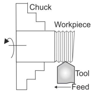
Fig. 5.12: Thread cutting
