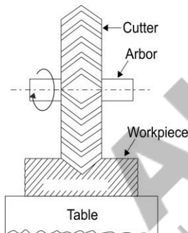
Fig. 5.26: Angular milling
