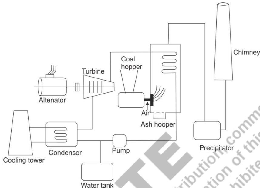
Fig. 2.20: Typical layout of a coal based thermal power plant
