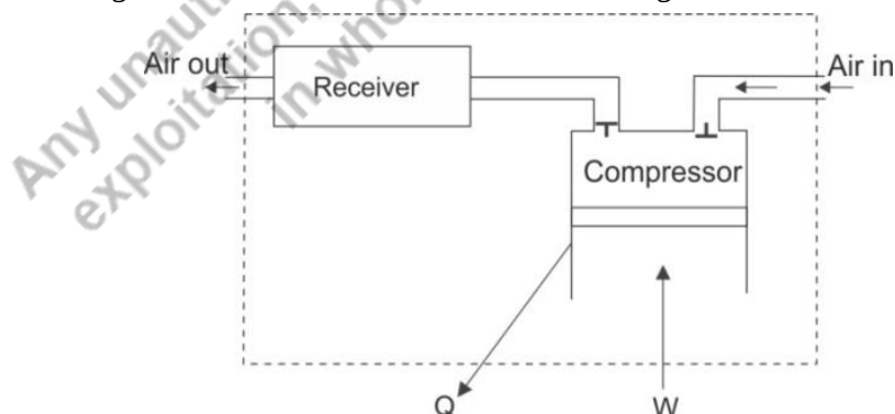
Fig. 1.20: Reciprocating compressor
