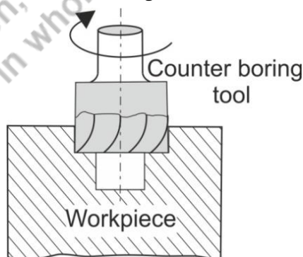
Fig. 5.37: Counter boring
