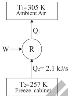
Fig. 1.41: System for example 1.13
