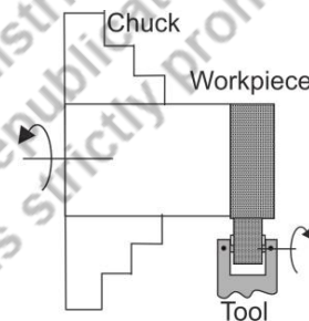
Fig. 5.10: Knurling
