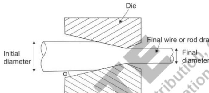
Fig. 4.20: Schematic of rod and wire process
