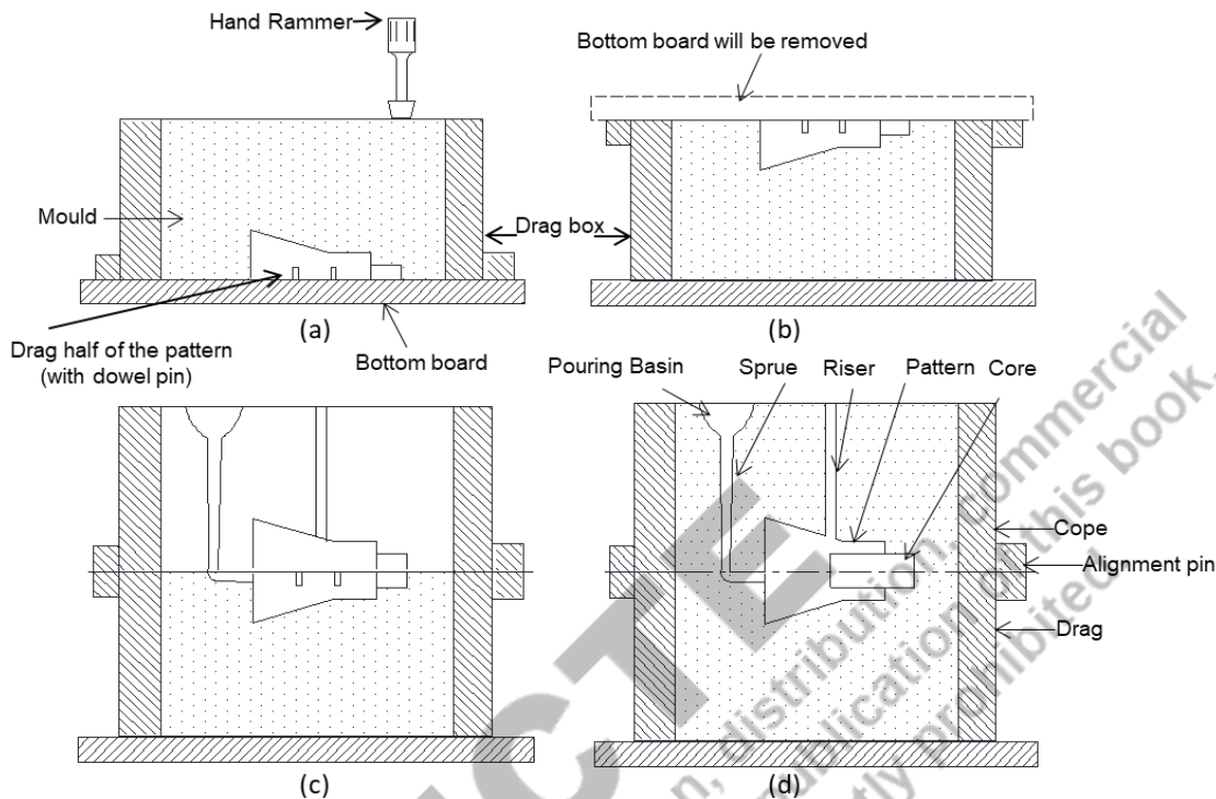
Fig.4.14: Schematic illustration of sand moulding process
