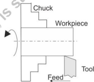
Fig. 5.6: Turning
