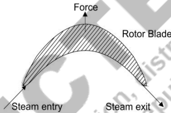
Fig. 3.1: Passage of steam through rotor blade section
