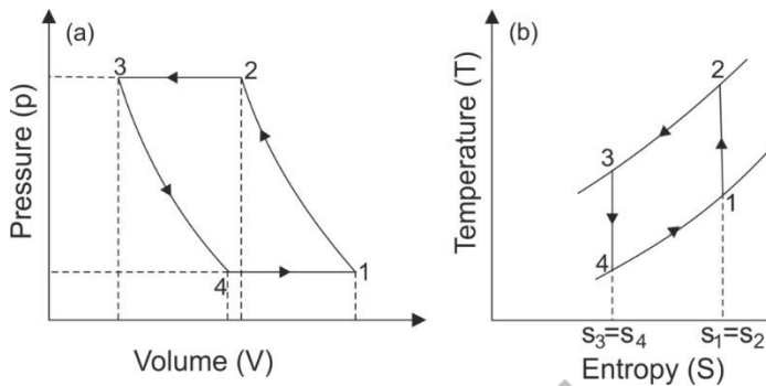
Fig. 3.26: (a) p-V plot, (b) T-s plot of Bell-Coleman cycle
