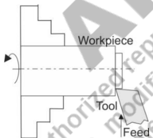
Fig. 5.5: Facing
