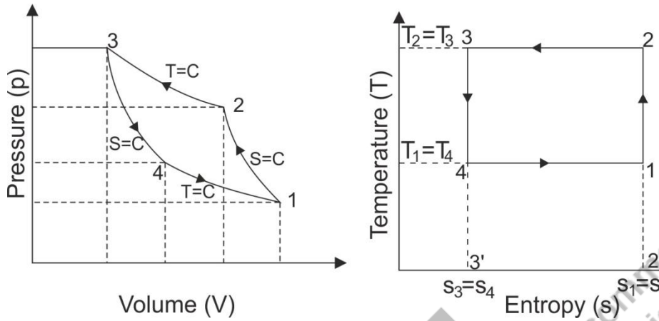
Fig. 3.24: p-V and T-s curve of Reversed Carnot cycle
